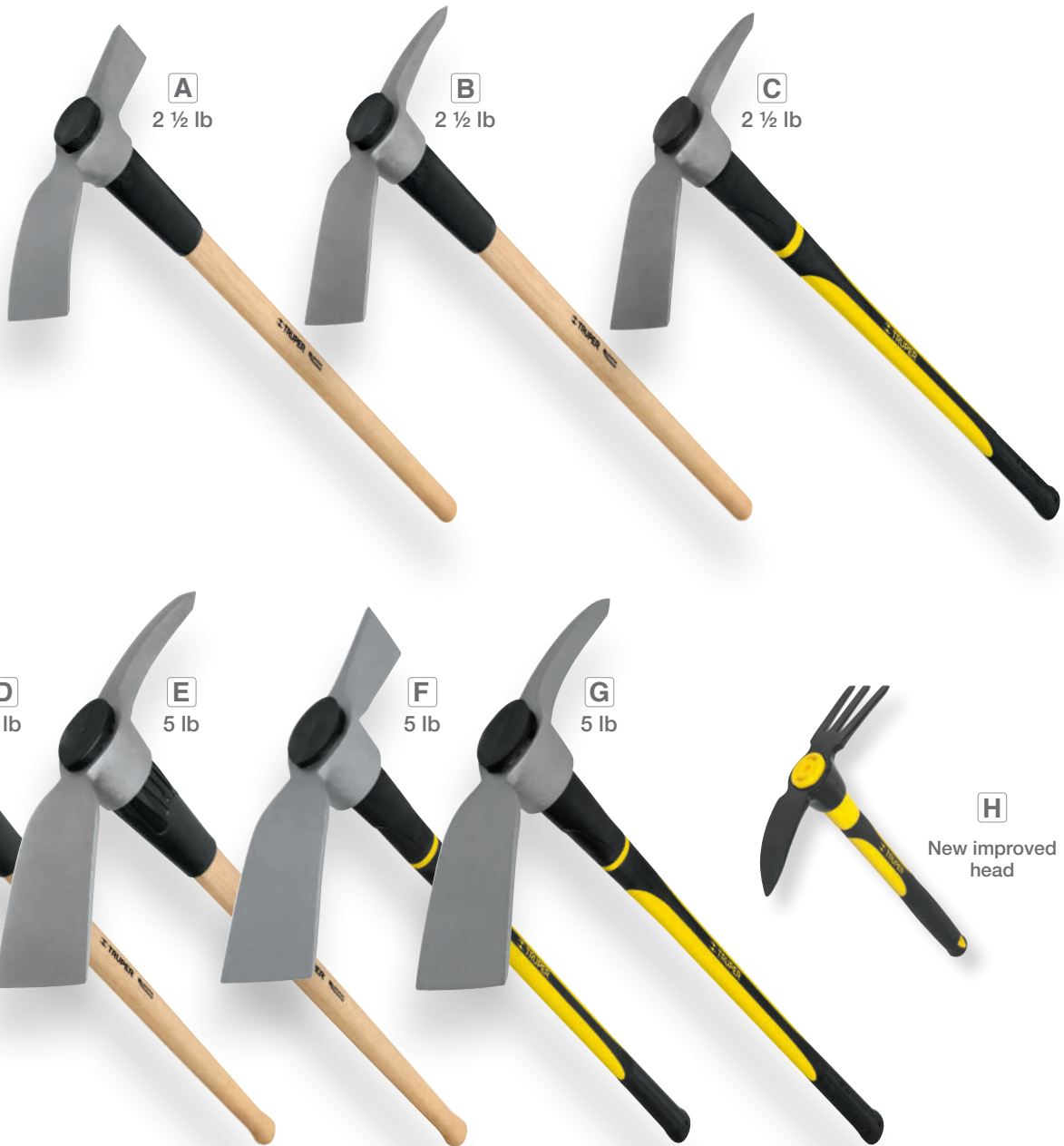
Wood handle with shock absorber poly guard
