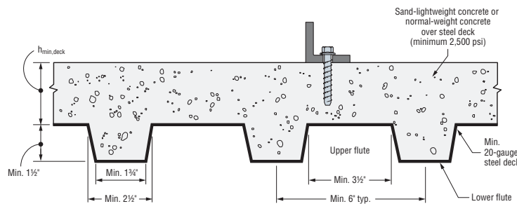
Figure 3. Installation of \frac{1}{4} "- and \frac{3}{8} "-Diameter Anchors in the Topside of Concrete over Metal Deck
