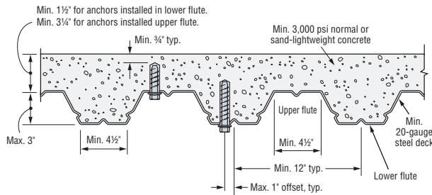
Figure 1. Installation of \frac{3}{8} "- and \frac{1}{2} "-Diameter Anchors in the Soffit of Concrete over Metal Deck
