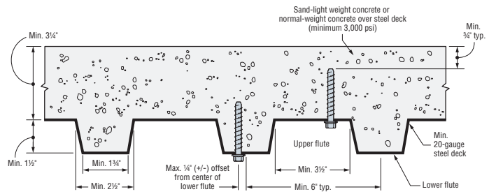
Figure 2. Installation of \frac{1}{4} "-Diameter Anchors in the Soffit of Concrete over Metal Deck
