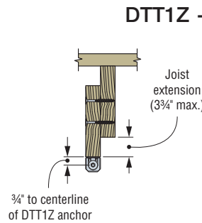
Figure 5B (end view)
