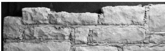
Leveling the top of each stone produces the best result as the Shale Stone units are irregular. Building up the mortar bed will be required to compensate for these variances, much the same as natural limestone, adding character to the overall appearance.
