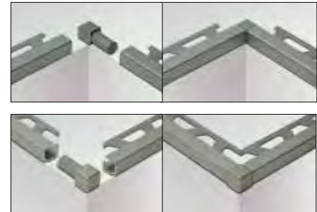
Inside/outside corner 90°/end cap
