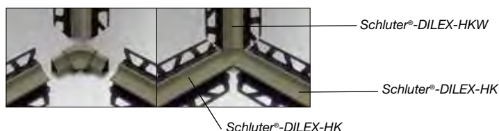
Inside corner, 3-way
