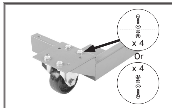
Figure 10. Fixed caster mounted to corner bracket.
