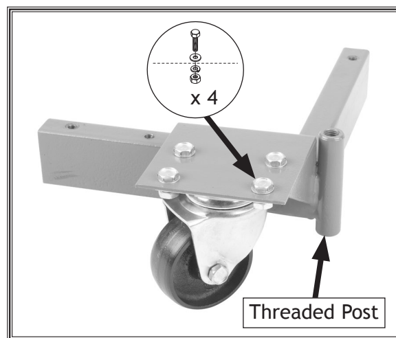
Figure 9. Swivel caster mounted to corner bracket with threaded post.
