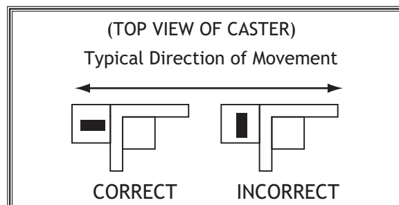
Figure 11. Mounting casters based upon typical direction of movement.
