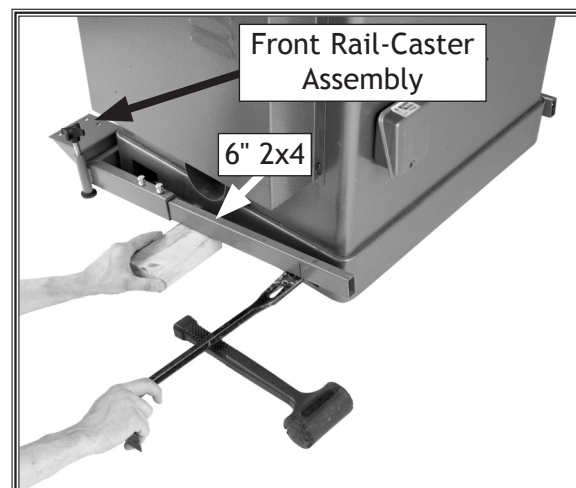
Figure 26. 2x4 placed under rail after using crowbar to raise rail up.
