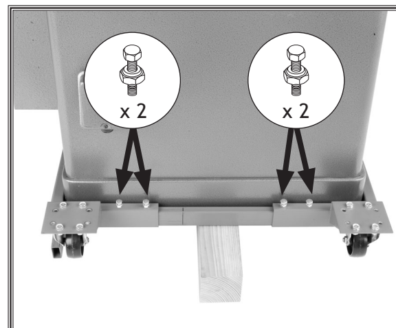
Figure 25. Rear rail fixed caster assembly secured.
