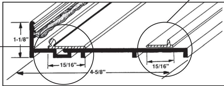
Inside Slider Installation
