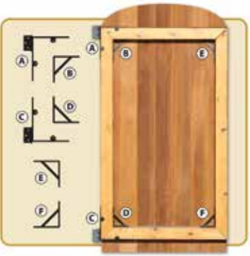
GCBHK01 Gate Corner Frame Brace and Hinge Kit UPC #664723101521
