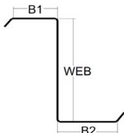
(Unsymmetrical Flange)
