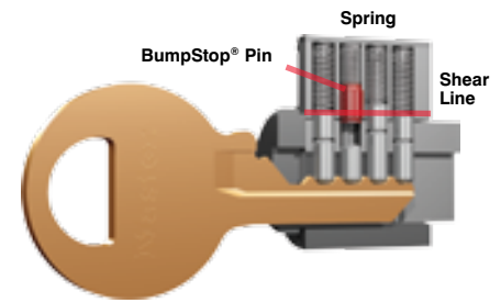
Master Lock Cylinder Cross-section
