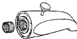
3/4" - 14 NPT THREAD
