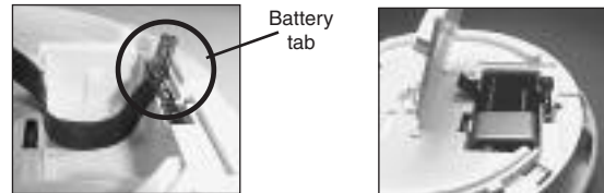
FIGURE 4 BATTERY REPLACEMENT
