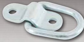
04521 1-1/2" D-Ring w/ Bracket, 2 Pack 300 lbs. WLL 900 lbs. Break Strength Package: Clamshell Ship Pack 6
