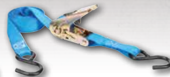
84518 15' x 1" Steel Ratchet Tie-Down 300 lbs. WLL 900 lbs. Break Strength
