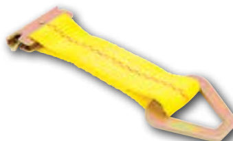
04316 7" x 2" E-Track Tie-Off Strap, Stamped D-Ring, 2 Pack 2,000 lbs. WLL 6,000 lbs. Break Strength Package: Clamshell Ship Pack 4
