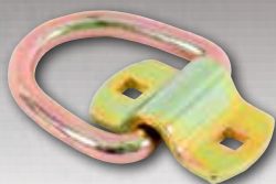
04529 3-3/8" D-Ring w/ Bracket, Bolt-On 3,666 lbs. WLL 11,000 lbs. Break Strength Package: Chip board Ship Pack 4
