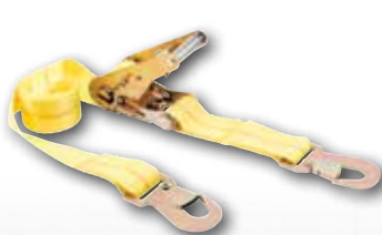
04105 7' x 2" Auto Ratchet Tie-Down w/Snap Hooks 2,000 lbs. WLL 6000 lbs. Break Strength Package: Clamshell Ship Pack 3
