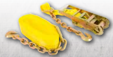
04655 30' x 3" Ratchet Tie-Down w/Chain Ends & Grab Hook 5,000 lbs. WLL 15,000 lbs. Break Strength
