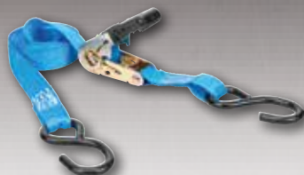
45518 15' x 1" Molded Ratchet Tie-Down 2 pack 500 lbs. WLL 1,500 lbs. Break Strength
