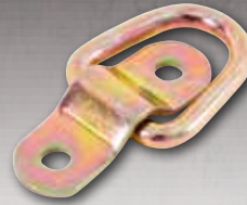
89311 1" D-ring w/ Bracket 400 lbs. WLL 1,200 lbs. Break Strength Package: Bulk/Cut Case Ship Pack 18
