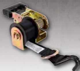
05530/ 89430 8' x 1-1/2" Rack-Ratchet®, Mountable 500 lbs. WLL 1,500 lbs. Break Strength
