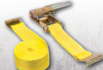
04637 27' x 3" Ratchet Tie-Down 5,000 lbs. WLL 15,000 lbs. Break Strength
