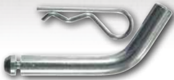
3015-008 Pin & Clip 5/8" Package: Chip board Ship Pack 6
