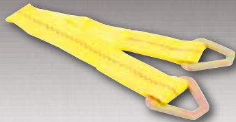
04224 24" x 2" Axle Strap w/D-Ring 3,333 lbs. WLL 10,000 lbs. Break Strength Package: Cardboard Sleeve Ship Pack 6
