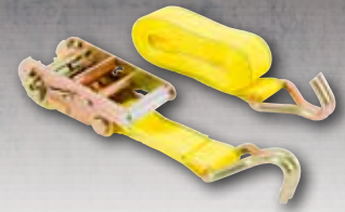
05522 15' x 1-3/4" Ratchet Tie-Down 1,666 lbs. WLL 5,000 lbs. Break Strength
