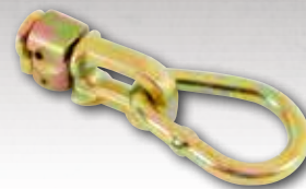
89304 O-Track Double Stud Fitting 2,000 lbs WLL 6,000 lbs. Break Strength Package: Bulk/Cut Case Ship Pack 12
