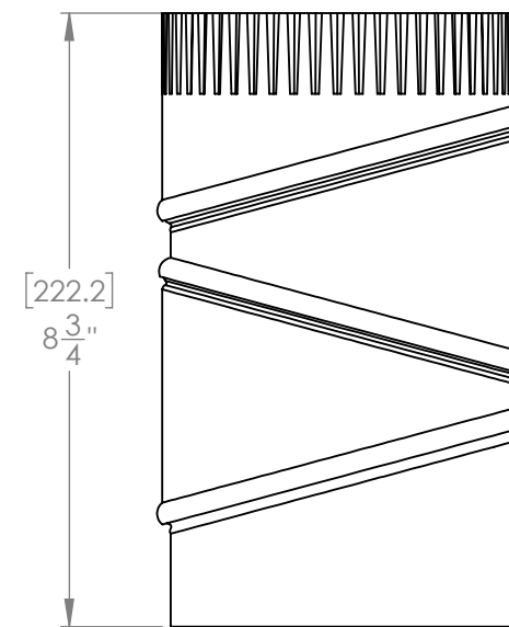
180 DEG POSITION
