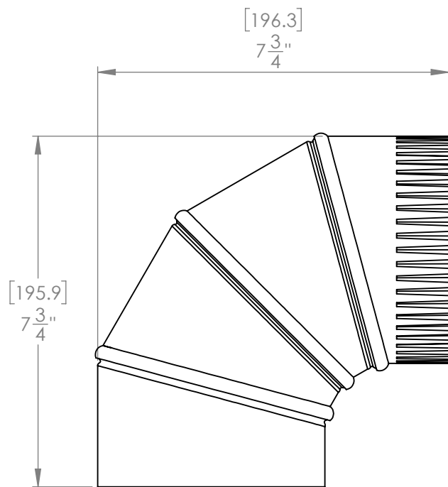
90 DEG POSITION
