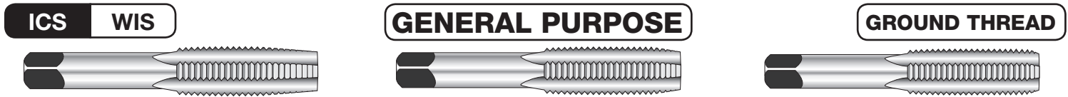
TAPER TAP (T) 7-10 Thread Chamfer at 5 degrees per side
