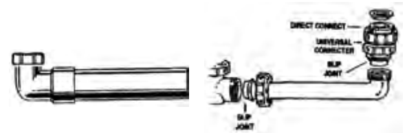
Waste Arm
