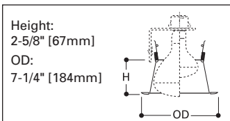
H930 R/PAR lamp aiming accessory for 310 and 426 trims. Allows 30° tilt and 358° rotation. 50W PAR30 max.
