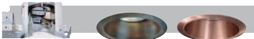
H930 R/PAR lamp aiming accessory for 310 and 426 trims. Allows 30° tilt and 358° rotation. 50W PAR30 max.
