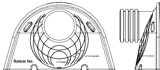
STORMASTER END CAP WITH PRE-FABRICATED STUBS @ TOP
