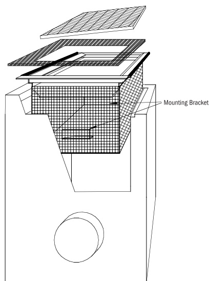
WALL MOUNT – COMBINATION INLET
