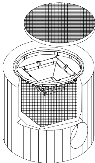
FRAME MOUNT – ROUND GRATED INLET
