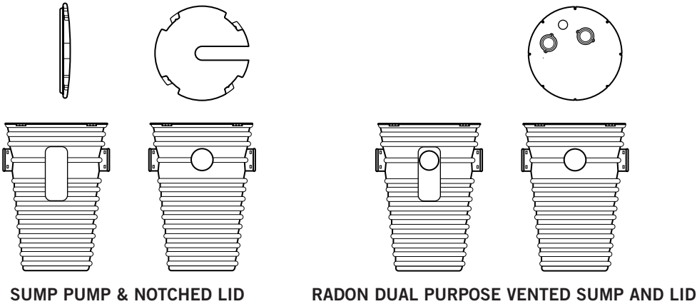
SUMP PUMP & NOTCHED LID
