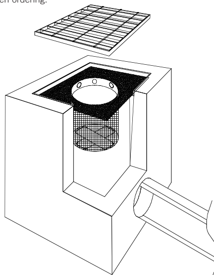
T-SERIES FRAME MOUNT
