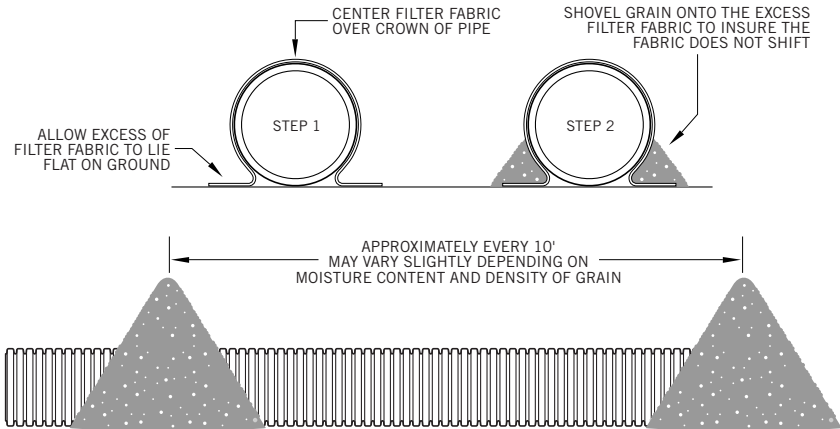
GRAIN-DRI PIPE
