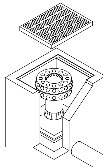
PERK FILTER – WALL MOUNT – FLAT GRATED INLET
