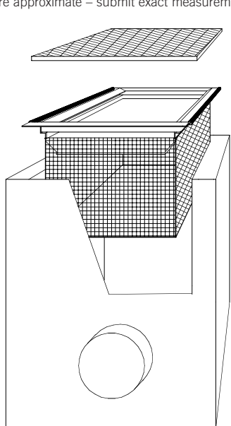
FRAME MOUNT – FLAT GRATED INLET
