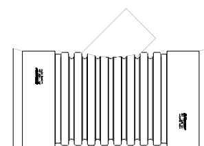
SURE-LOK BELL-AND-SPIGOT & SURE-LOK WT
