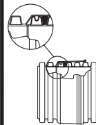
10"-18" (250-450mm) BLUE SEAL BELL-AND-SPIGOT
