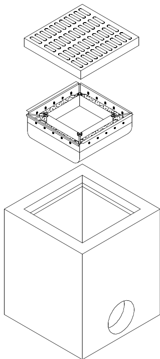
FRAME MOUNT – FLAT GRATED INLET – SHALLOW INSTALLATIONS
