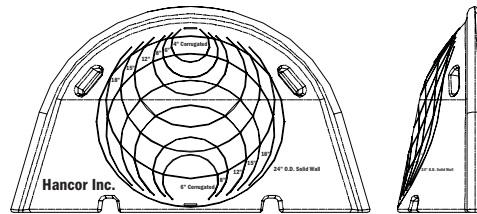
STORMASTER SOLID END CAP
