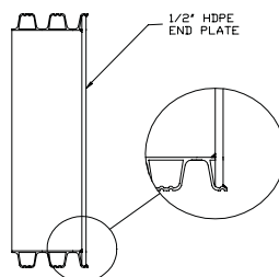
WELDED END PLATE ON HEADER
