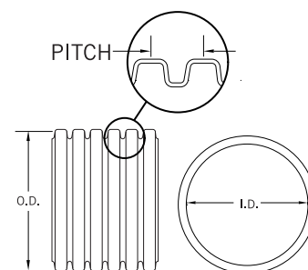
CO-EX PIPE
