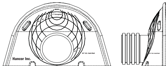
STORMASTER END CAP WITH PRE-FABRICATED STUBS @ BOTTOM
