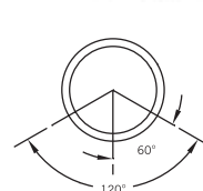
Option 1: 3 Hole, 120°
