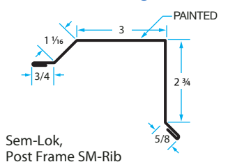
EF-1 Gable Flashing
