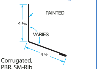
EW-1 Endwall Flashing
