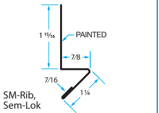
BD-1 Base Drip
