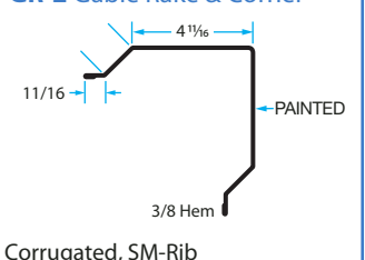
GR-2 Gable Rake & Corner
