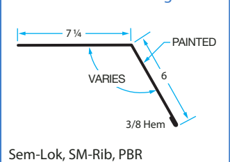
GF-1 Gambrel Flashing
