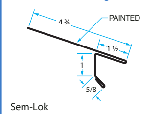
ED-2R Eave Flashing
