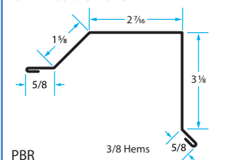
GR-7 Gable Rake
