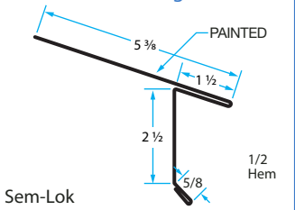
ED-2 Eave Flashing
