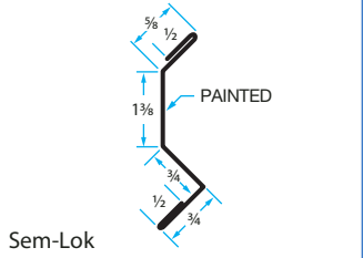
CF-1 Counter Flashing
