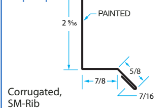
DC-1 Drip Cap
