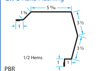
GR-5 Rake Flashing
