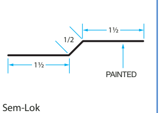
CL-2 Cleat Offset
