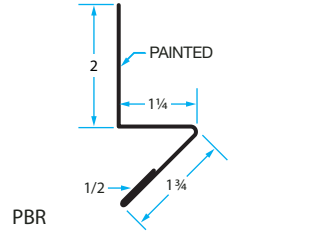
BD-2 Base Drip: 2 inch
