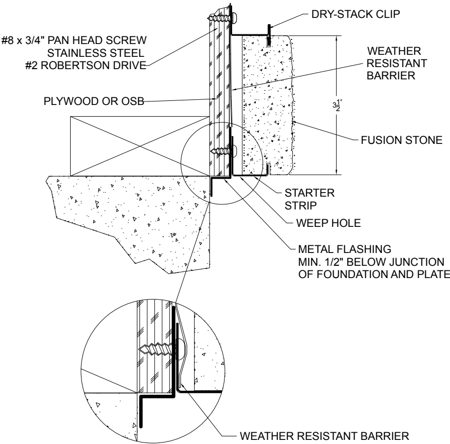
Typical Cross Section of Veneer Mounting System
