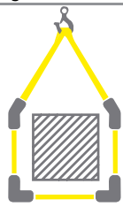
BASKET HITCH
