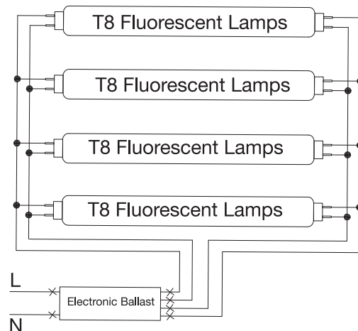
Electronic Ballast Type with Four Lamps
