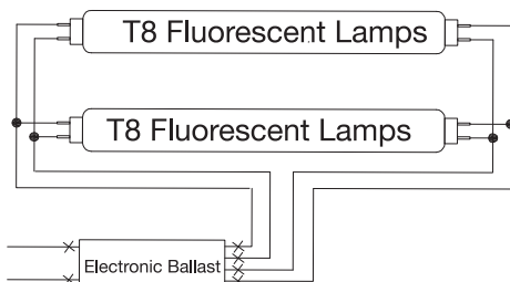
Electronic Ballast Type
