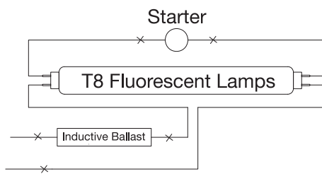
Inductive ballast type
