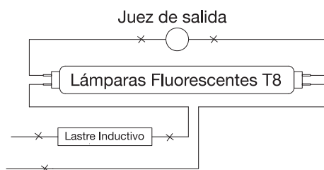
Inductive ballast type
