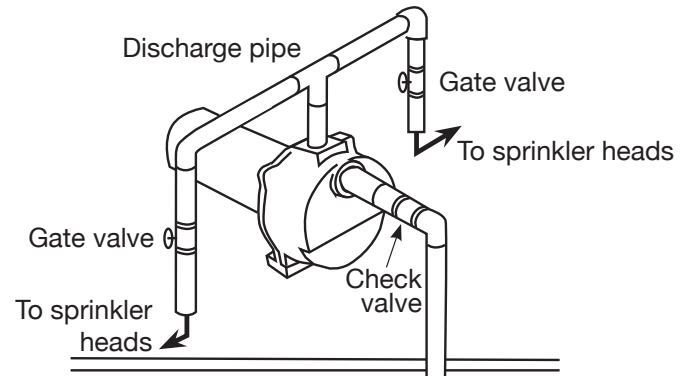
Figure 2 Driven point installation, multiple well points
