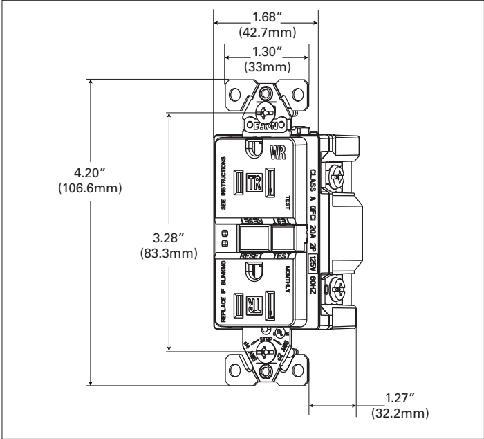
Figure 2. TWRSGF15 Line art with dimensions
