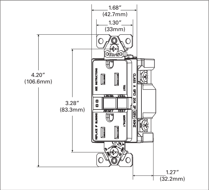
Figure 3. SGF15, SGF15-M & SGF15F Line art with dimensions
