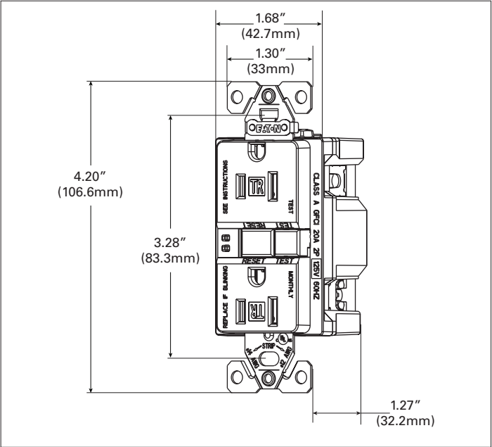
Figure 4. TRSGF15, TRSGF15-M & TRSGF15F Line art with dimensions
