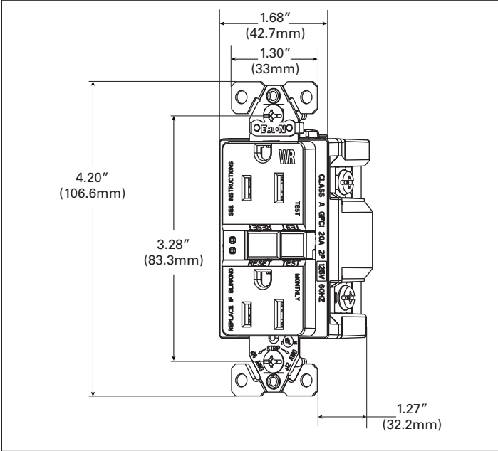
Figure 1. WRSF15 Line art with dimensions
