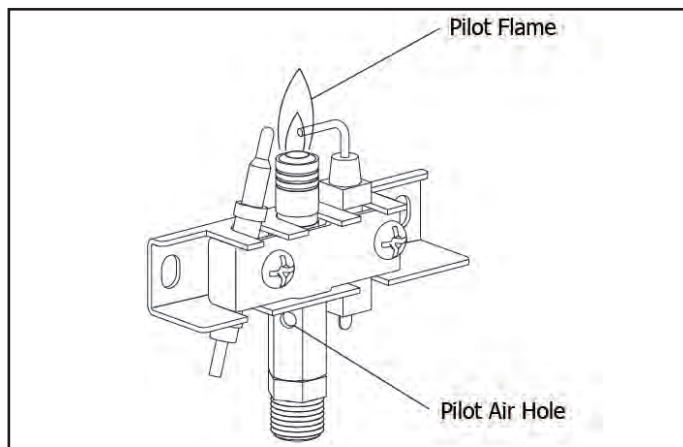
Fig. 5 - Pilot Assembly
