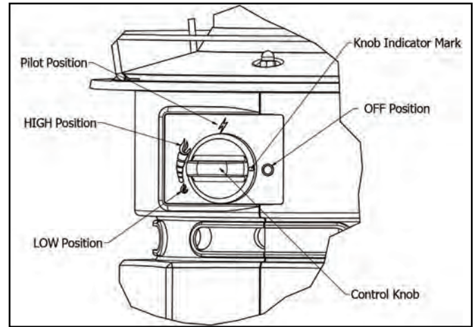
Fig. 2 - Lighting Instruction
