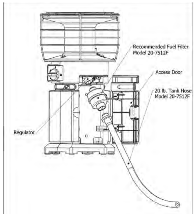
Fig. 1a - Remote Tank Installation
