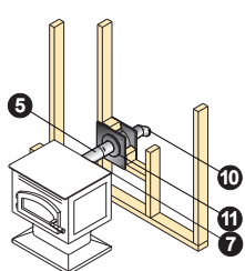
Through-The-Wall
