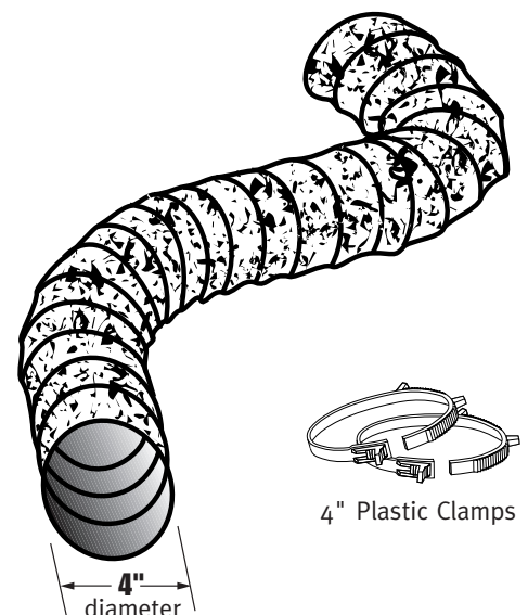
Supurr-Flex ® UL LISTED Clothes Dryer Transition Duct
