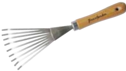
35-1805 Stainless Steel Shrub Rake 5-Year Warranty Head: 7"L x 4.5"W; Total: 13"L; .35lbs
