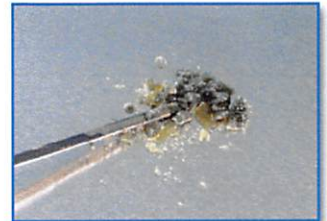
Polymer-based leak stops can harden (as shown above) within the air conditioning or refrigeration system, causing significant damage to components.
