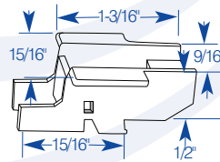
Top Guide w/ Wings
