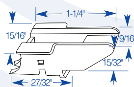
Top Guide w/ Wings
