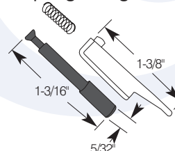
Flip Type Spring Plunger
