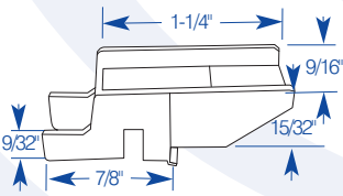
Top Guide w/o Wings
