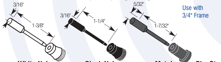
Snap-In Spring Plunger
