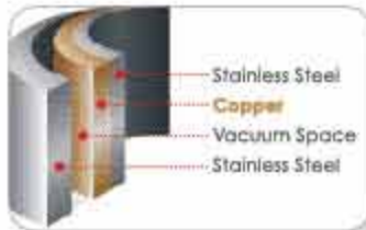
Triple-wall vacuum seal
