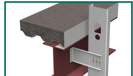
Extended Fast Clip™ Installation
