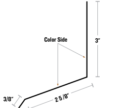
DORMER FLASHING
