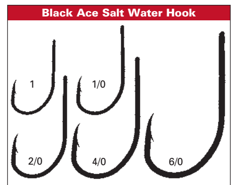
3111 (Black) O'Shaughnessy bend, beak point, 2X-short shank, straight-eye, forged, reversed Uses: Saltwater, Salmon and Steelhead Flies
