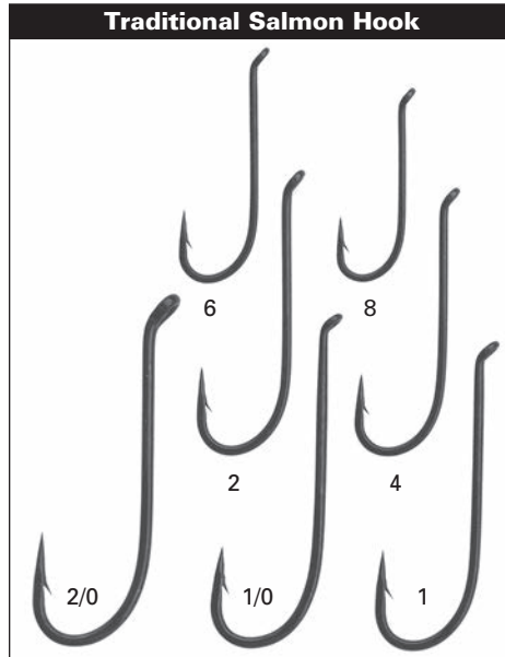
2441 (Black) Tapered-loop up-eye, 1X-heavy wire, forged Uses: Classic Atlantic Salmon Wet Flies, Hairwing Salmon/Steelhead Flies
