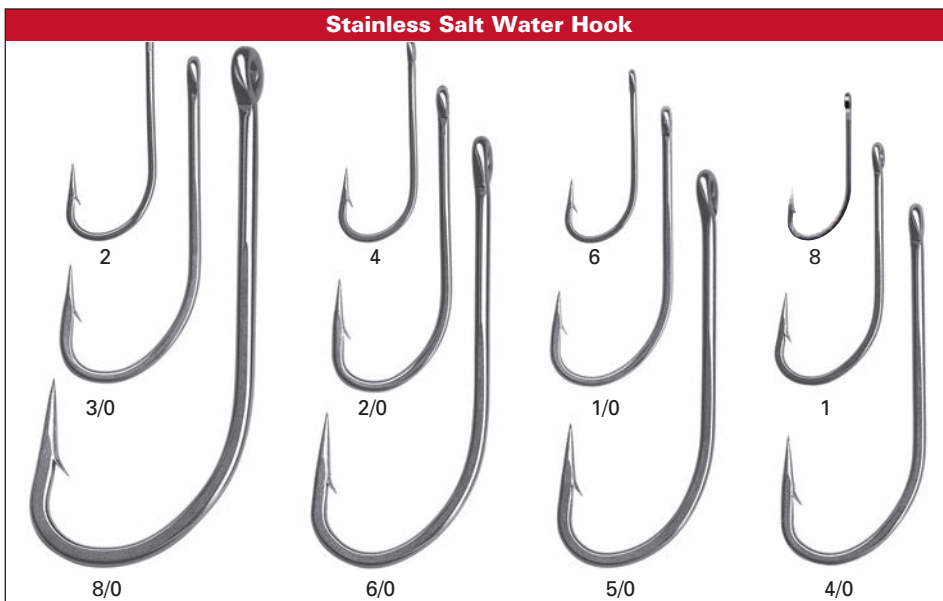
2546 (Stainless Steel) O'Shaughnessy bend, straight eye, forged, stainless steel, ground needle point Uses: Salt Water Fly Patterns. Size 8 commonly used for Crab & Shrimp Patterns
