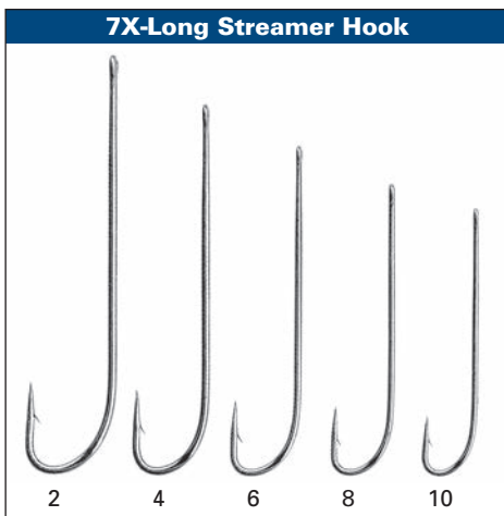
2370 (Bronze) Modified Limerick bend, tapered-loop eye, 3X-heavy wire, 7X-long shank Uses: Classic Streamers
