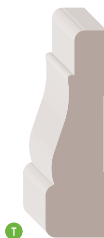
OW356 11/16" x 2-1/4"
