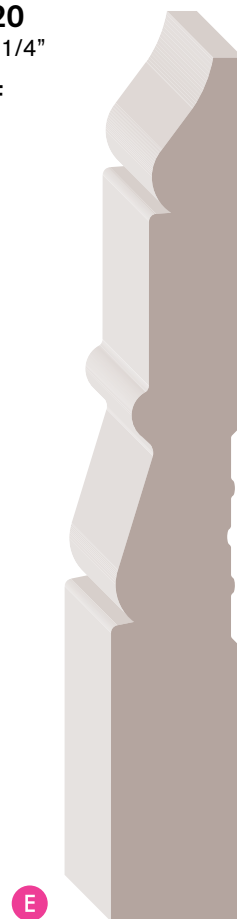
04312 11/16" x 4-1/2"
