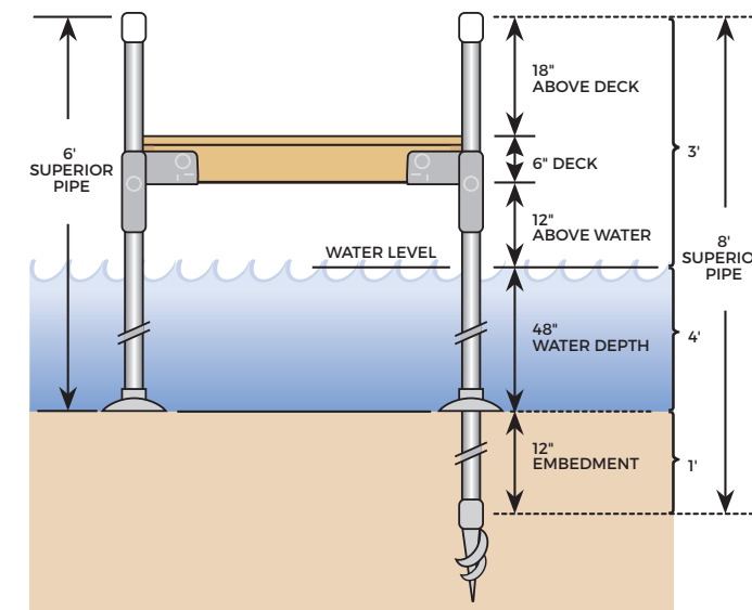
TYPICAL TOMMY DOCKS SETUP
