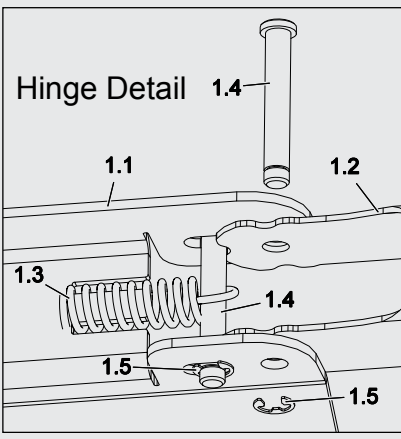
#5281003 2-Nozzle Boom Assembly
