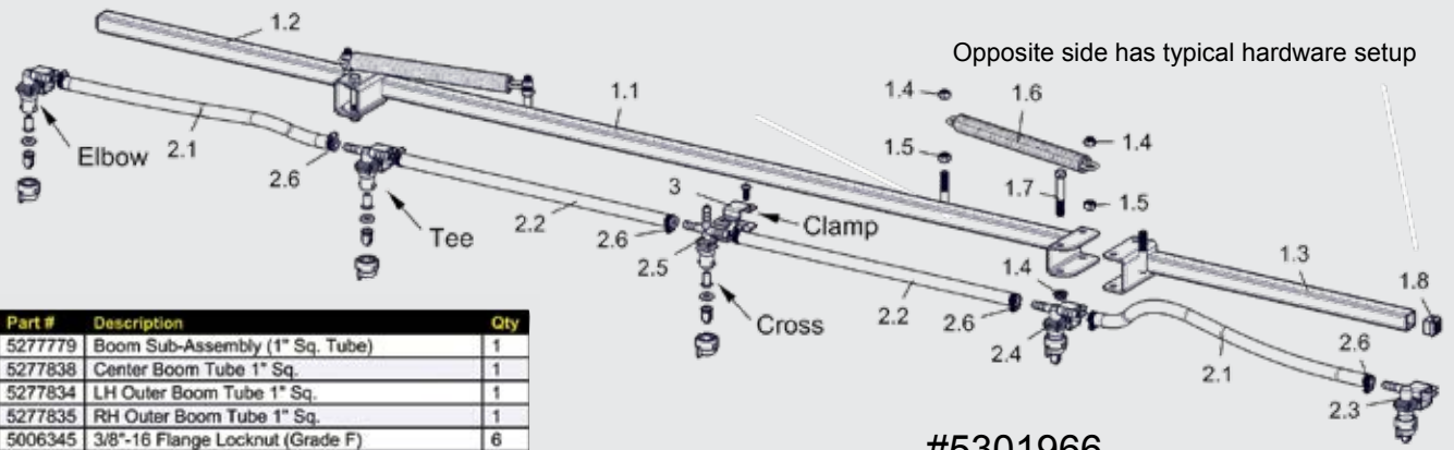
#5301966 5-Nozzle Boom Assembly
