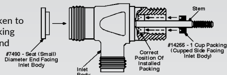
How To Install #7490 - Valve Seat And Replace #14255 - 1 Cup Packing
